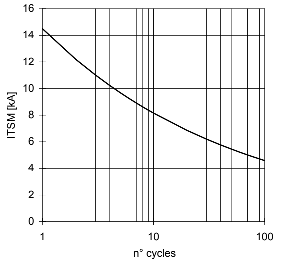
SURGE CHARACTERISTIC T_j = 125^\circ\text{C}
