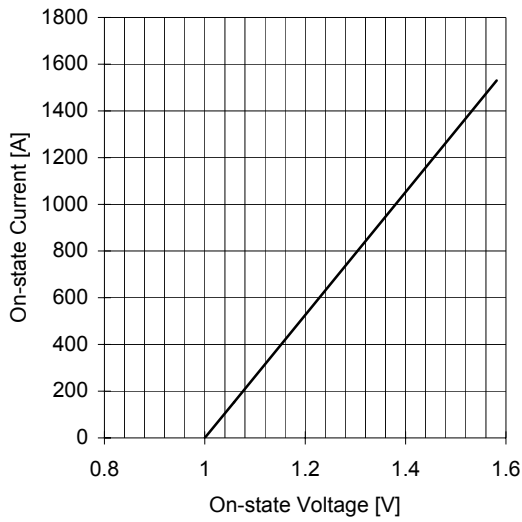
ON-STATE CHARACTERISTIC T_j = 125^\circ\text{C}
