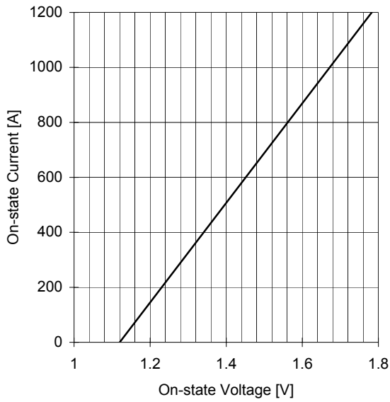
ON-STATE CHARACTERISTIC T_j = 125^\circ\text{C}
