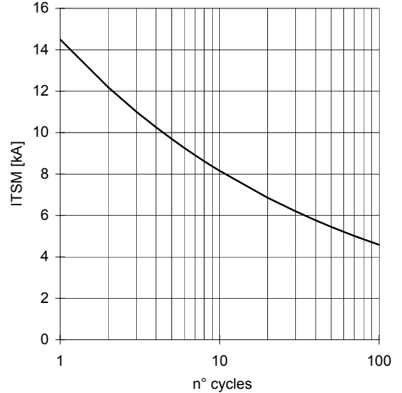
SURGE CHARACTERISTIC T_j = 135\text{ }^\circ\text{C}
