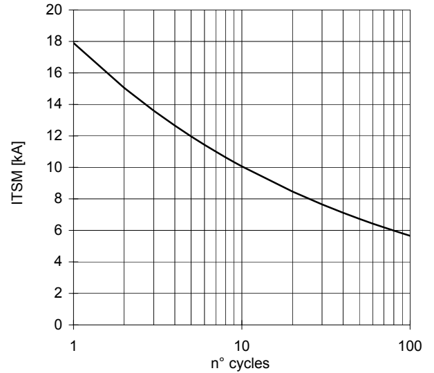
SURGE CHARACTERISTIC T j = 150 °C
